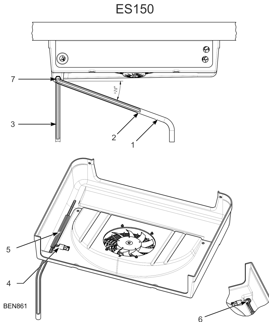
Figure 12. ES-150 Rear and Bottom views
